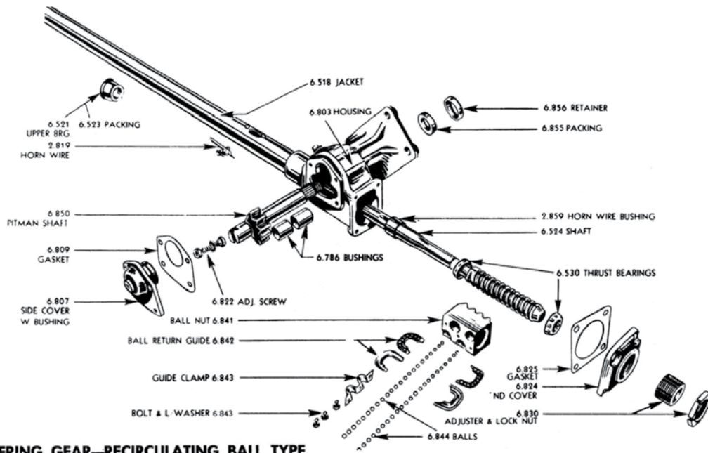
1941-46 STEERING GEAR—RECIRCULATING BALL TYPE
