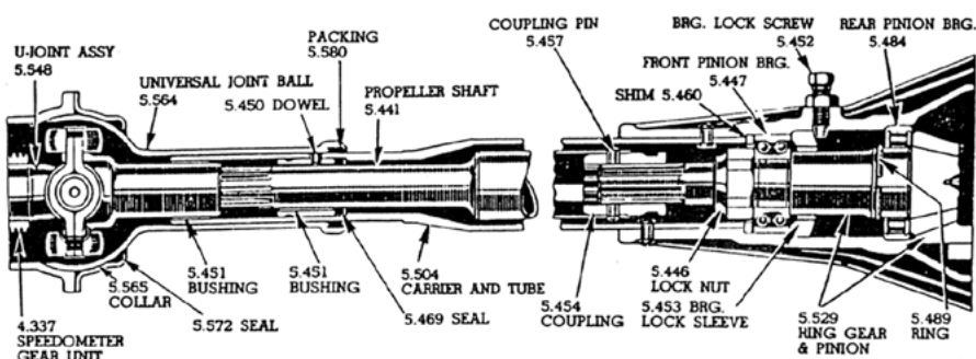
PROPELLER SHAFT AND HOUSING—PASSENGER CAR
