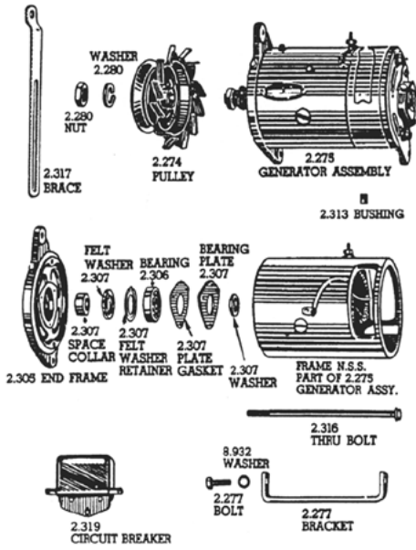
GENERATOR
