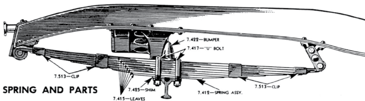
REAR SPRING AND PARTS
