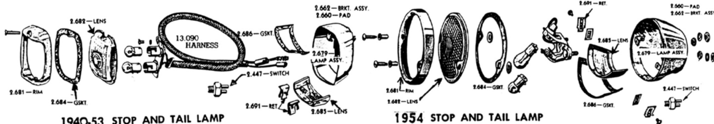
1940-53 STOP AND TAIL LAMP
