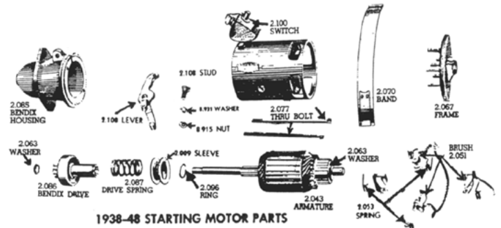
1938-48 STARTING MOTOR PARTS
