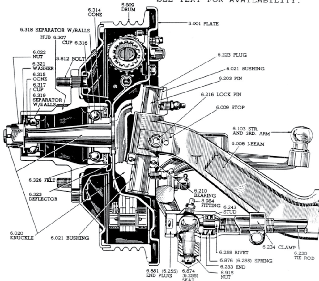
FRONT AXLE—CONVENTIONAL TRUCK (EXC. HVY. DUTY)
