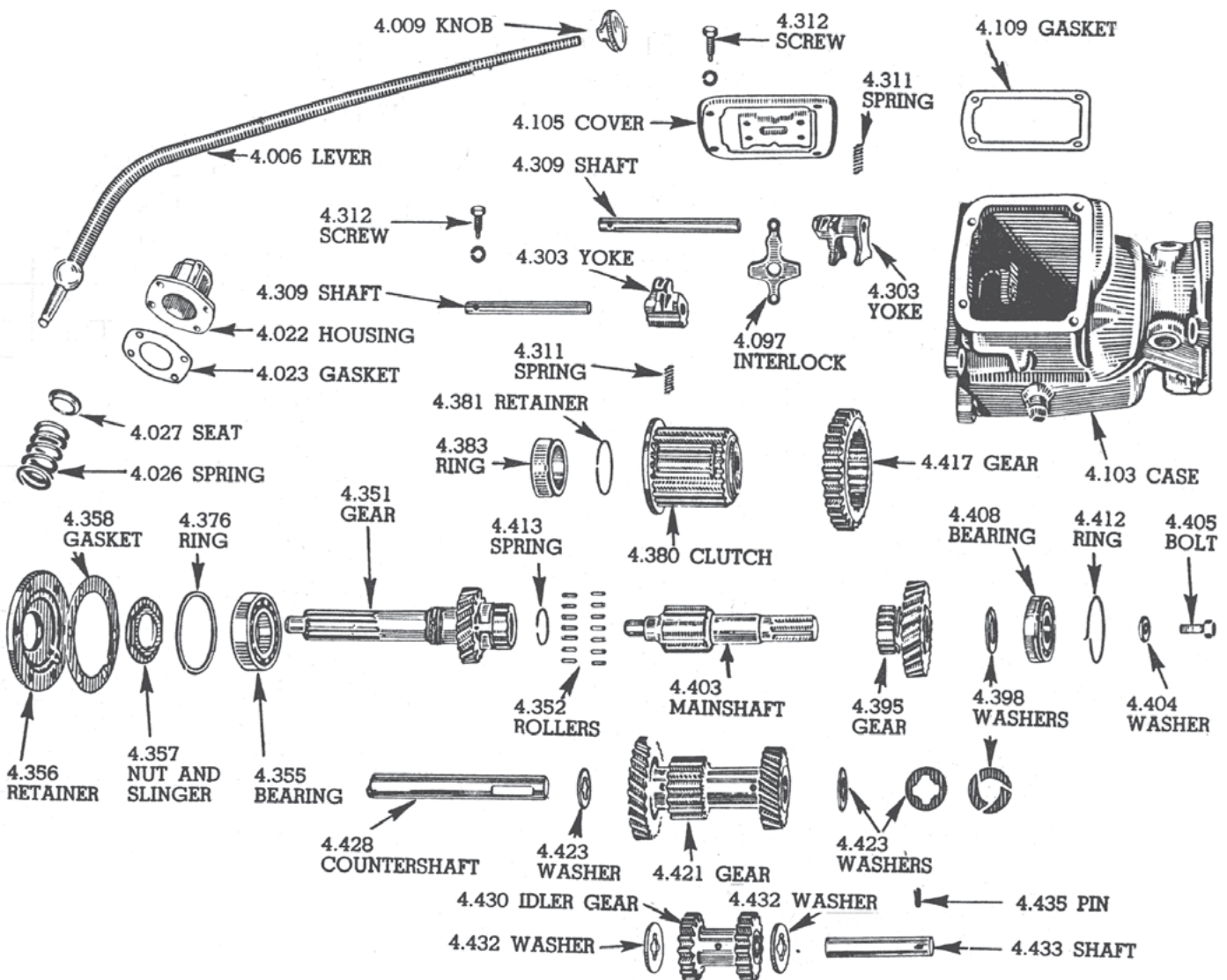
1937-47 SYNCHRO-MESH TRANSMISSION (CENTER GEARSHIFT)
