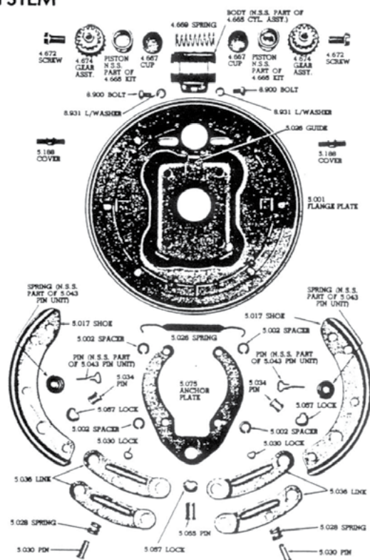
HYDRAULIC BRAKE PARTS—FRONT
