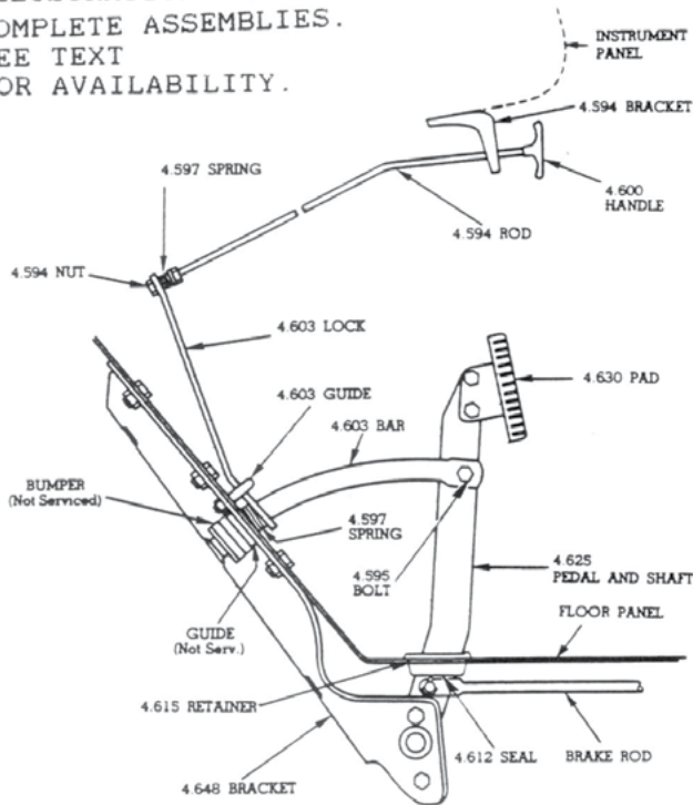
TRUCK PARKING BRAKE CONTROLS (FOOT OPER.)
