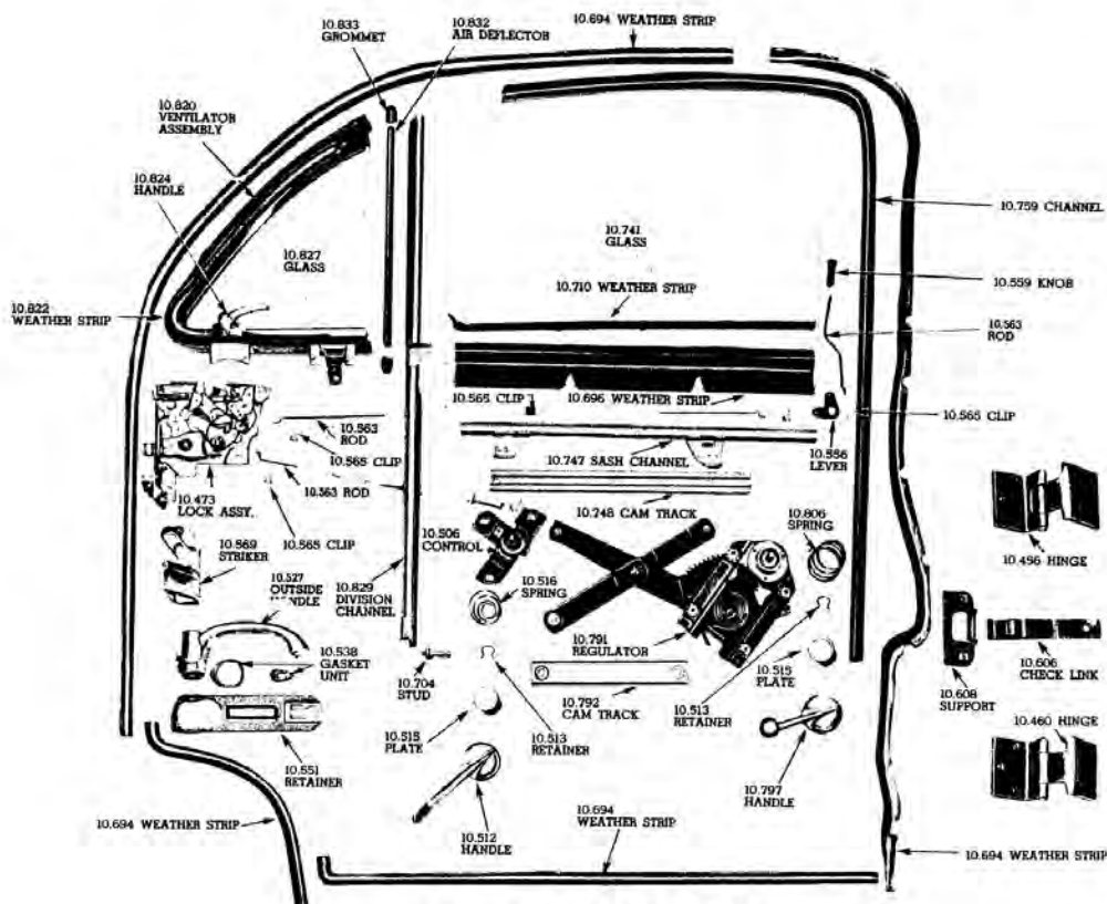
1949-52 REAR DOOR PARTS
