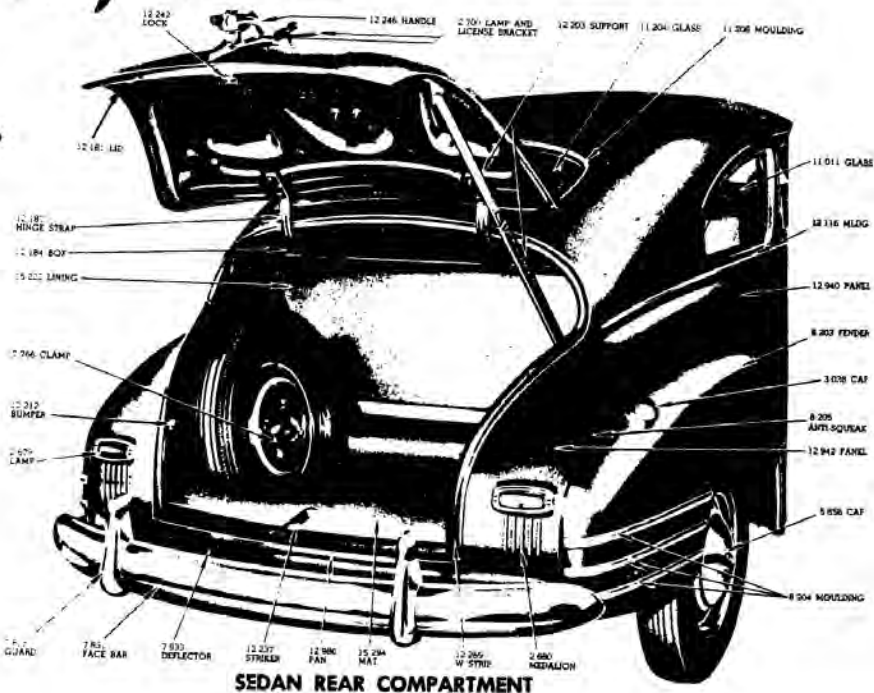
SEDAN REAR COMPARTMENT
