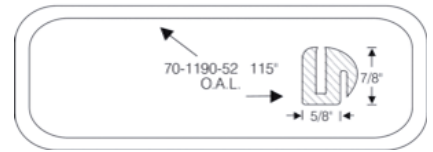
Vulc. Fixture VU-11
