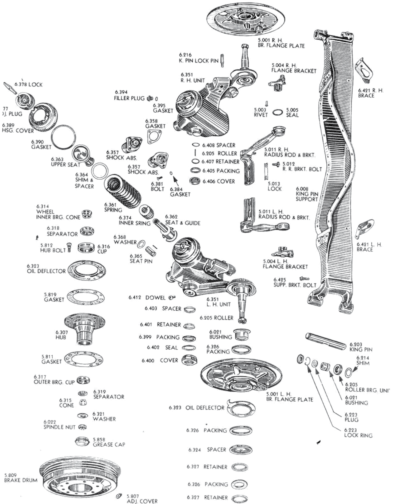
KNEE ACTION PARTS—ENCLOSED TYPE
