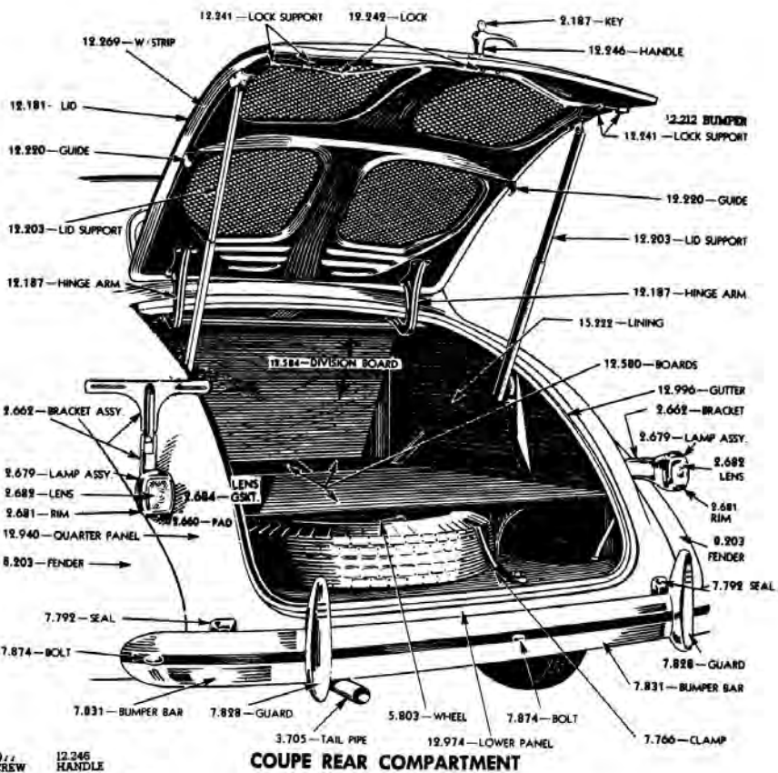
COUPE REAR COMPARTMENT
